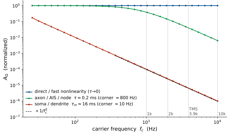
Figure S4: Somatic demodulation dies at kHz, but a fast element survives (Jansen–Rit, open-loop detector). Open-loop demodulated response (normalized to the \tau \rightarrow 0 value) vs. carrier frequency up to 10 kHz. With direct coupling ( \tau \rightarrow 0 ) the response is flat—carrier-independent. A slow somatic membrane ( \tau_m \approx 16 ms) rolls off as 1/f_c^2 (dashed guide), killing kHz demodulation; a fast element (axon/AIS/node, \tau \approx 0.2 ms) retains an appreciable response into the kHz band ( \sim 0.14 at 2 kHz, \sim 0.04 at the TMS peak 3.9 kHz). The same membrane filter attenuates TMS at the soma, which is why neither TMS nor TI should be thought of as driving the soma at kHz.
