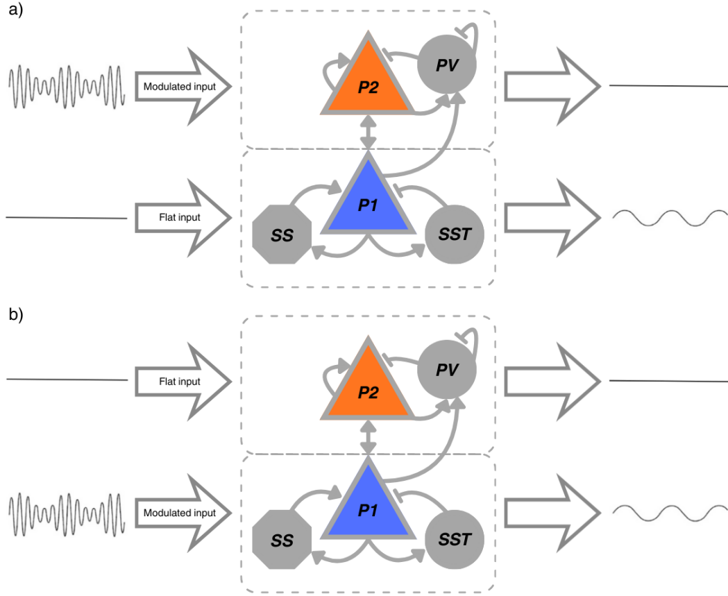
Figure S1: Stimulation setup in a LaNMM column. The column couples a superficial PING sub-circuit (pyramidal P_2 + PV ; gamma) and a deep JR sub-circuit (pyramidal P_1 + SS + SST ; alpha). (a) the TI field drives P_2 while P_1 receives a flat drive; (b) the TI field drives P_1 while P_2 is flat. Through the sigmoid nonlinearities and P_1 – P_2 coupling, the generated beat-frequency component is transferred to the deep loop: P_2 carries the modulated fast carrier, while P_1 exposes the recovered low-frequency component (right traces).
