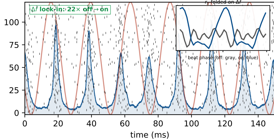
(d) Entrained, TI ON ( \Delta f=42 Hz): gamma bursts gate to the TI beat
