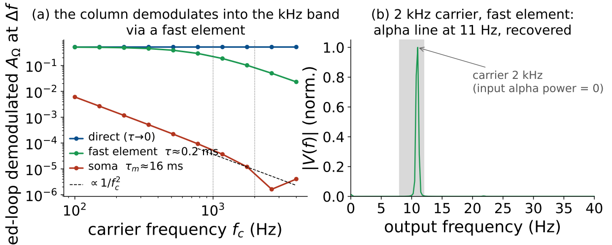
Figure S12: Demodulation at a genuine kHz carrier (Jansen–Rit, closed loop). The applied field passes through an explicit membrane filter before the sigmoid. (a) Closed-loop demodulated A_\Omega at \Delta f = f_0 vs. carrier f_c for three coupling routes: direct ( \tau \rightarrow 0 , carrier-independent), fast element (axon/AIS/node, \tau \approx 0.2 ms; survives into the kHz band), and soma ( \tau_m \approx 16 ms; collapses as 1/f_c^2 ). (b) Output spectrum for a 2 kHz carrier delivered through the fast element: a clean alpha line at f_0 , synthesized by the column although the input carries no alpha power.
