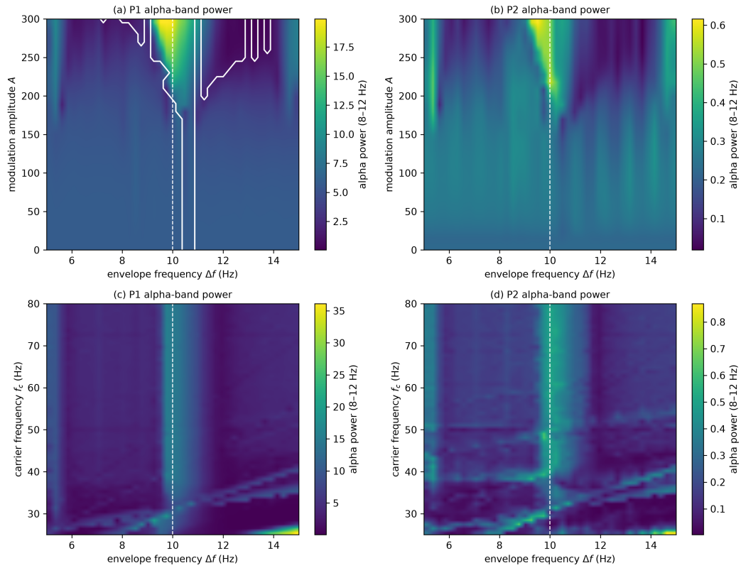
Figure S10: LaNMM Arnold tongues: AM input delivered directly to the deep P_1 (alpha) loop. (a,b) Alpha power of P_1 and P_2 vs. amplitude A and \Delta f . (c,d) Alpha power vs. carrier frequency and \Delta f : P_1 responds across a broad carrier band (a vertical ridge at \Delta f \approx 10 Hz)—carrier-independent, the direct-coupling limit of Eq. (10).
