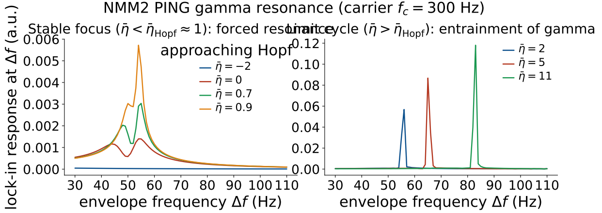
Figure 8: NMM2 PING gamma resonance (exact mean field). Lock-in response of the excitatory rate r_E at the envelope frequency \Delta f under an AM field (carrier 300 Hz). Left (stable focus, \bar{\eta} < \bar{\eta}_{\text{Hopf}} \approx 1 ): forced resonance at the gamma frequency ( f_0 \approx 55 Hz), growing as the Hopf is approached ( 1/\gamma gain), with the resonant frequency rising with \bar{\eta} . Right (limit cycle, \bar{\eta} > \bar{\eta}_{\text{Hopf}} ): entrainment of the autonomous gamma. The input carries no power at \Delta f ; the response is synthesized by the exact quadratic v^2 nonlinearity.
