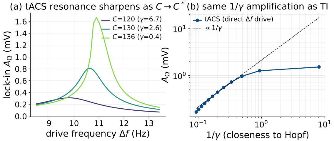
Figure S4: tACS shares the network amplifier (Jansen–Rit). A direct low-frequency (tACS) drive at \Delta f enters the column without a carrier, so it needs no demodulation, but feeds the same near-Hopf resonator. With the operating point pinned, sweeping the coupling C (= J) toward the alpha Hopf: (a) the lock-in resonance at \Delta f sharpens and grows as C \rightarrow C^* ; (b) the response grows as 1/\gamma (dashed) and saturates near criticality—the same network amplification as the demodulated TI drive (Fig. 9), but linear in the field rather than square-law. Throughout, the column is a stable focus ( \gamma > 0 ).
