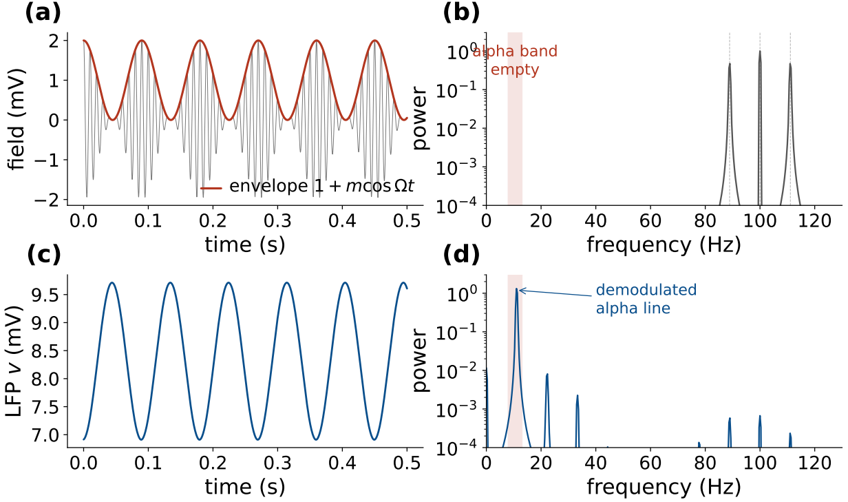
Figure 3: An alpha rhythm is synthesized from a carrier-only input (Jansen–Rit below Hopf). (a) The AM field s(t) and its envelope. (b) The input spectrum has lines only at f_c and f_c \pm \Delta f (89, 100, 111 Hz); the alpha band (shaded) is empty. (c) The output v = y_1 - y_2 oscillates at the envelope frequency. (d) The output spectrum has a strong peak at \Omega \approx 11 Hz, synthesized by the sigmoid and absent from the input.
