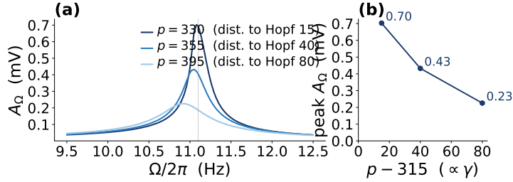
Figure 4: The recovered envelope drives a resonance that sharpens toward the Hopf (Jansen–Rit). Fixed-point regime ( p > 315 , stable focus): lock-in response at \Omega vs. envelope frequency ( \varepsilon = 0.3 mV). (a) The demodulated drive forces a Lorentzian resonance at f_0 \approx 11.1 Hz whose peak redshifts slightly as the damping grows ( \omega_{\text{peak}} = \sqrt{\omega_0^2 - 2\gamma^2} ; 11.08 \rightarrow 10.93 Hz across the three curves); the response carries no power at \Omega in the absence of drive, so this is genuine forced gain. (b) The peak height grows as the Hopf is approached ( p \rightarrow 315 , distance to Hopf \rightarrow 0 ). Three points cannot establish a power law; the 1/\gamma scaling is quantified over a decade, together with its saturation, in Fig. 9(c). The complementary above-Hopf regime, where the demodulated drive entrains the autonomous alpha within a 1:1 Arnold tongue, is characterized with the appropriate observable (output frequency f_{\text{out}} , not lock-in amplitude) in Fig. S5.
