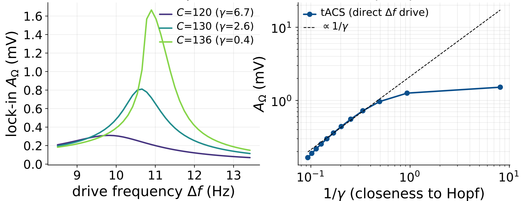
(a) tACS resonance sharpens as C \rightarrow C^* (b) same 1/\gamma amplification as TI
