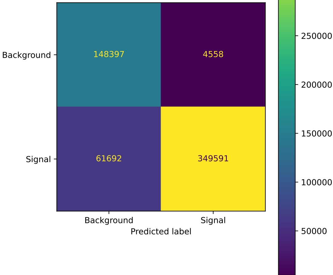
Confusion matrix (threshold = 0.16)
