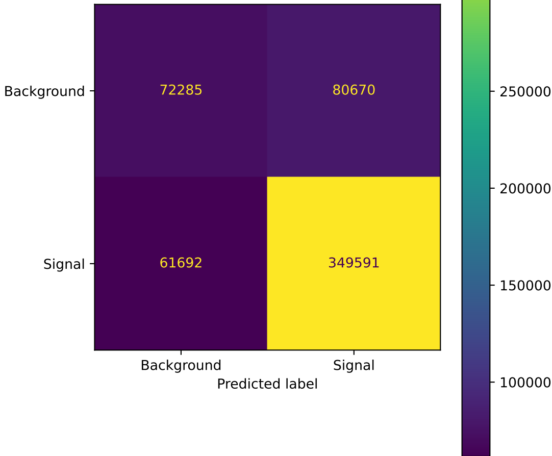
Confusion matrix (threshold = 0.14)
