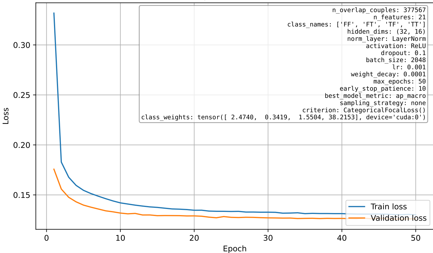
Training and validation loss
