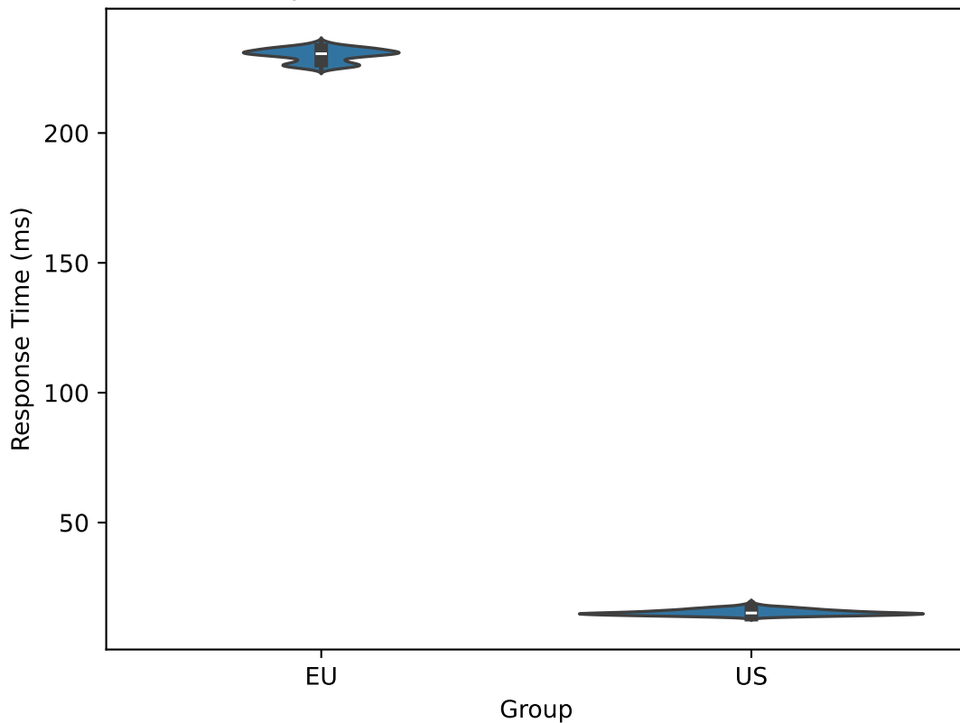
APP Response Times - 1 Core in US - both workers
