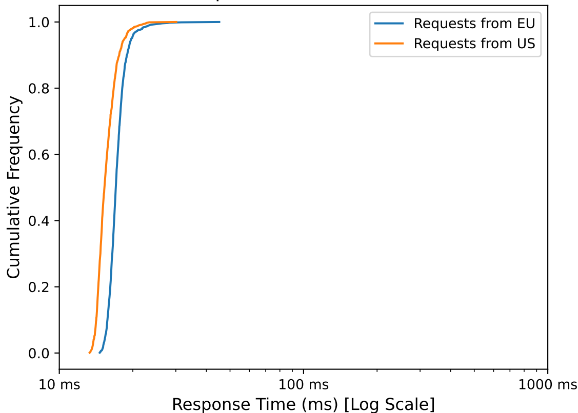
Response Time CDF - APP
