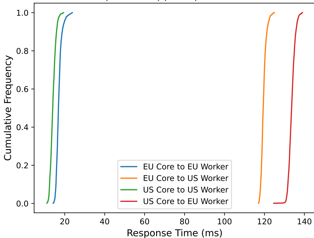
99p CDF - App Response Time
