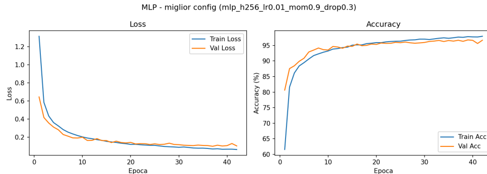
Curve MLP
