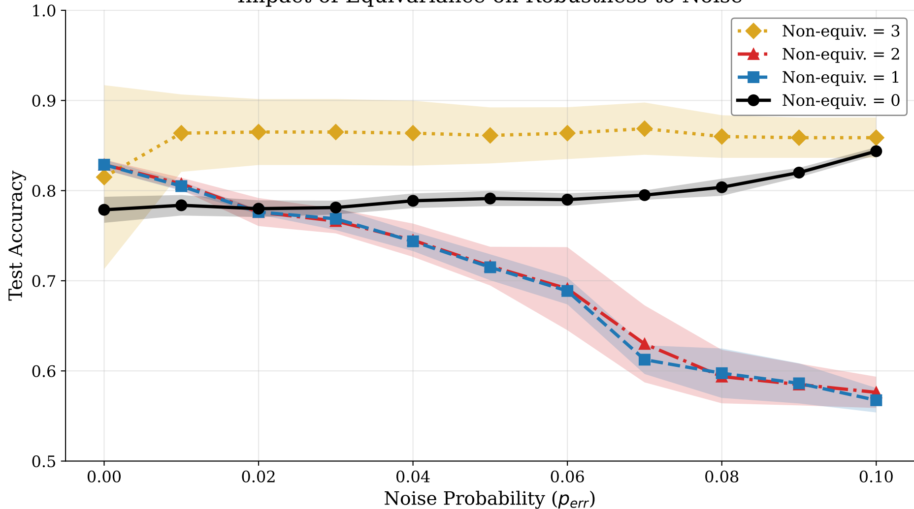
Impact of Equivariance on Robustness to Noise
