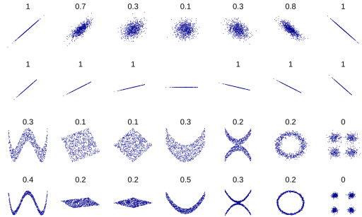
Distance correlation
