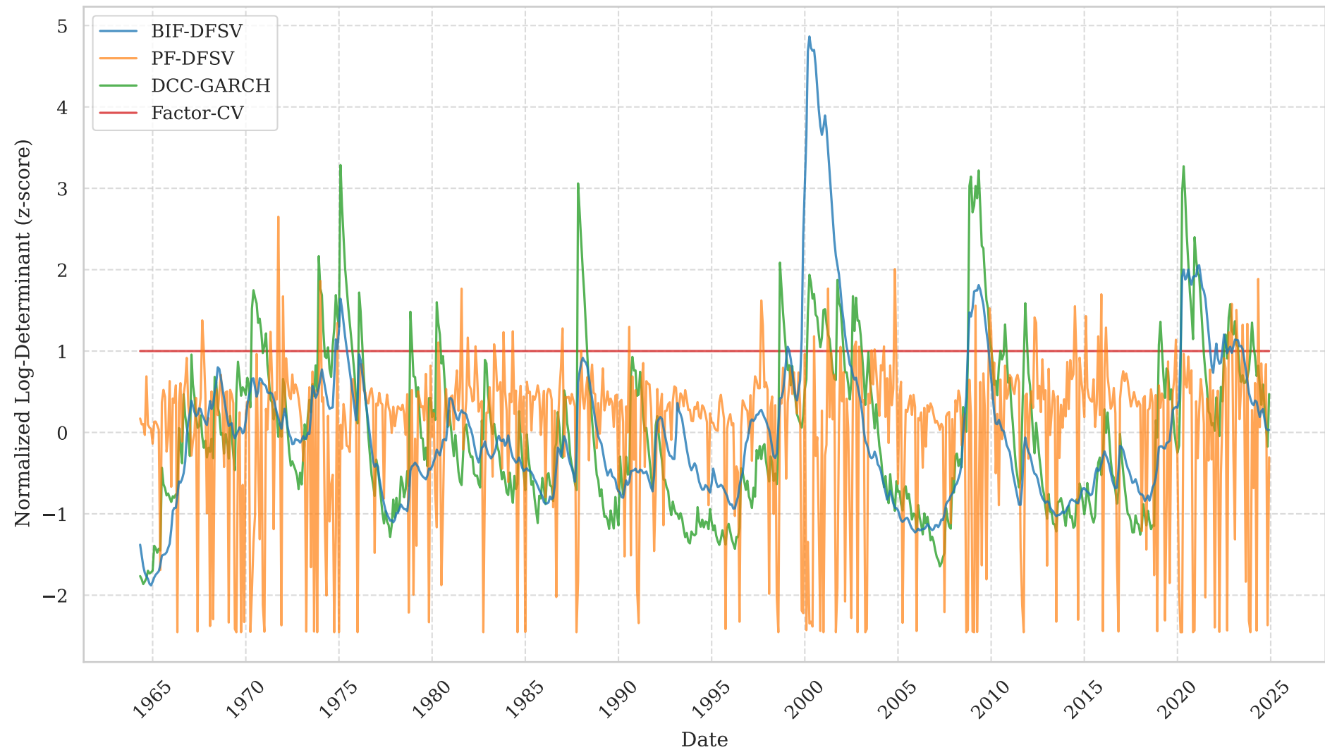
Normalized Log-Determinant of Conditional Covariance Matrices
