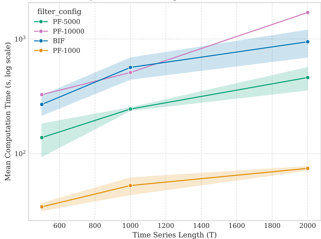
Computation Time Scaling vs. T (Fixed N=10, K=3)
