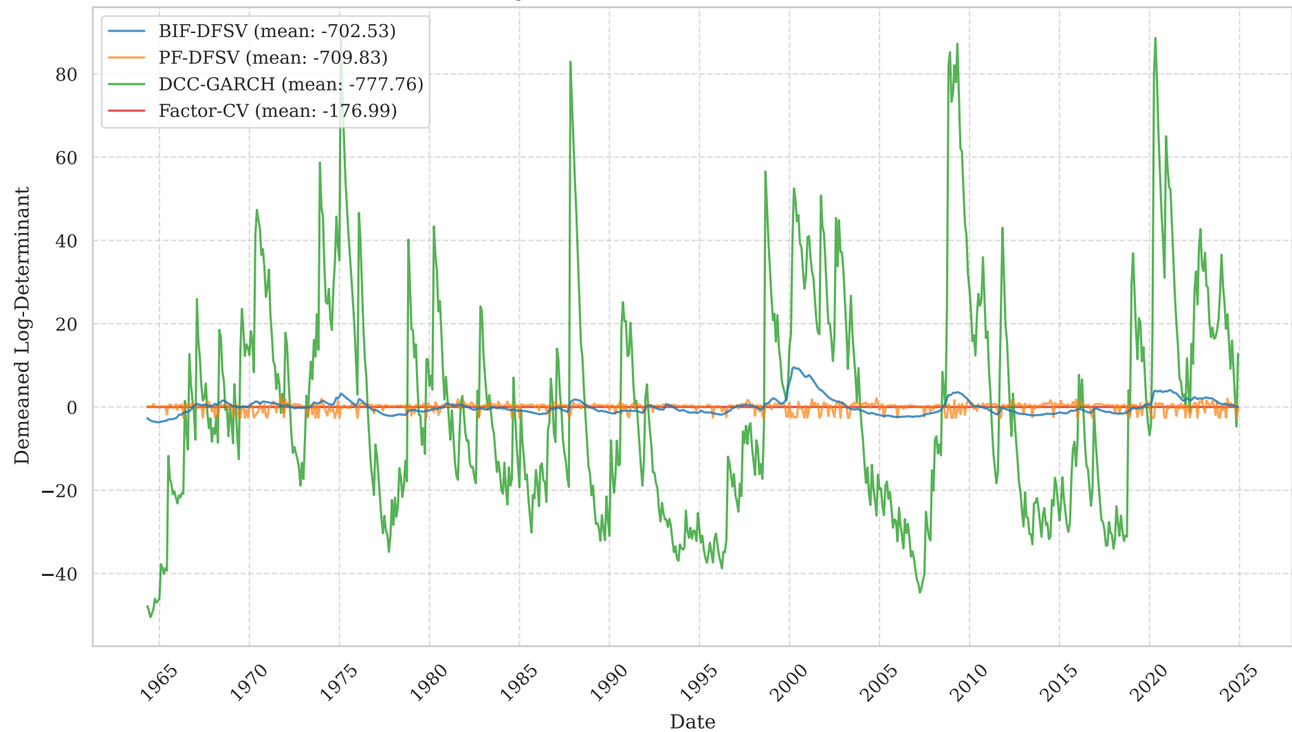
Demeaned Log-Determinant of Conditional Covariance Matrices
