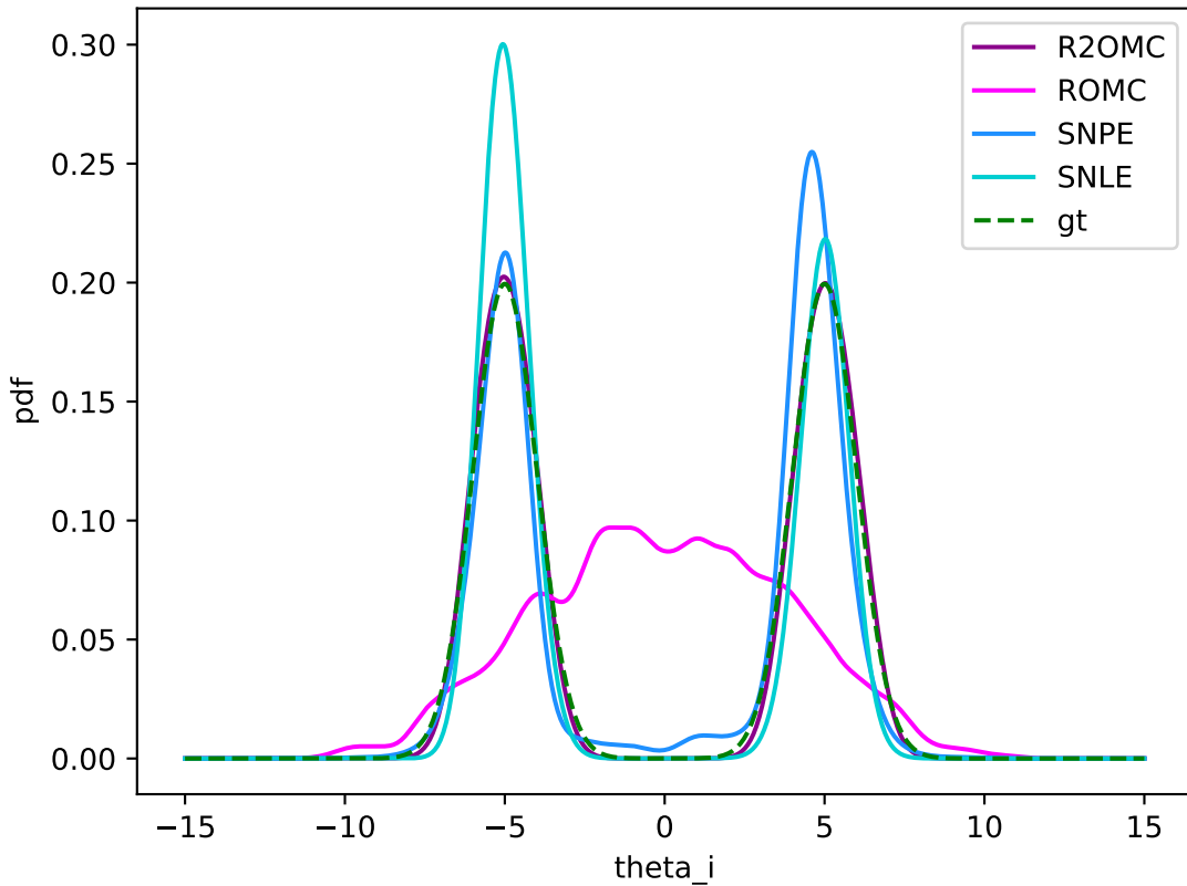
IID observations
