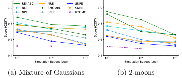
Figure 7: SBI benchmark: performance (C2ST) vs compute budget (log number of simulator runs).
