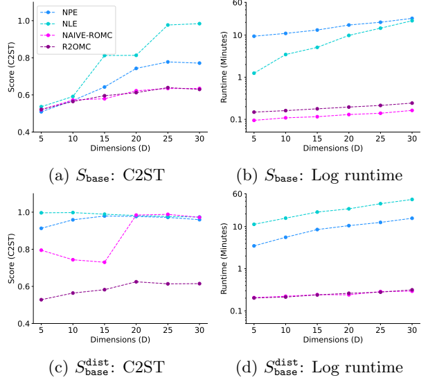
Figure 3: Base simulator, varying dimensionality.
