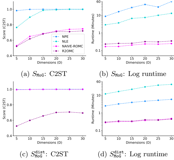
Figure 4: MoG simulator, varying dimensionality.
