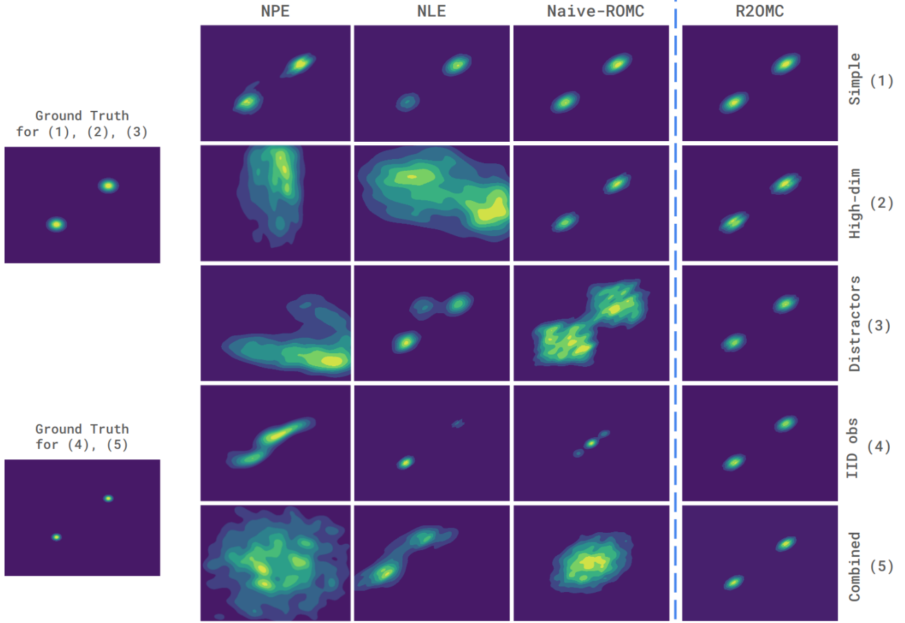
Figure 1: The simple setup (1) shows two-dimensional marginals for a five-dimensional inference problem, the high-dimensional setup (2) the same for a 20-dimensional problem. Distractors (3) add 10 uninformative dimensions to (1). (4) extends (1) to four iid observations. (5) combines (2-4). Details in Appendices A and B.
