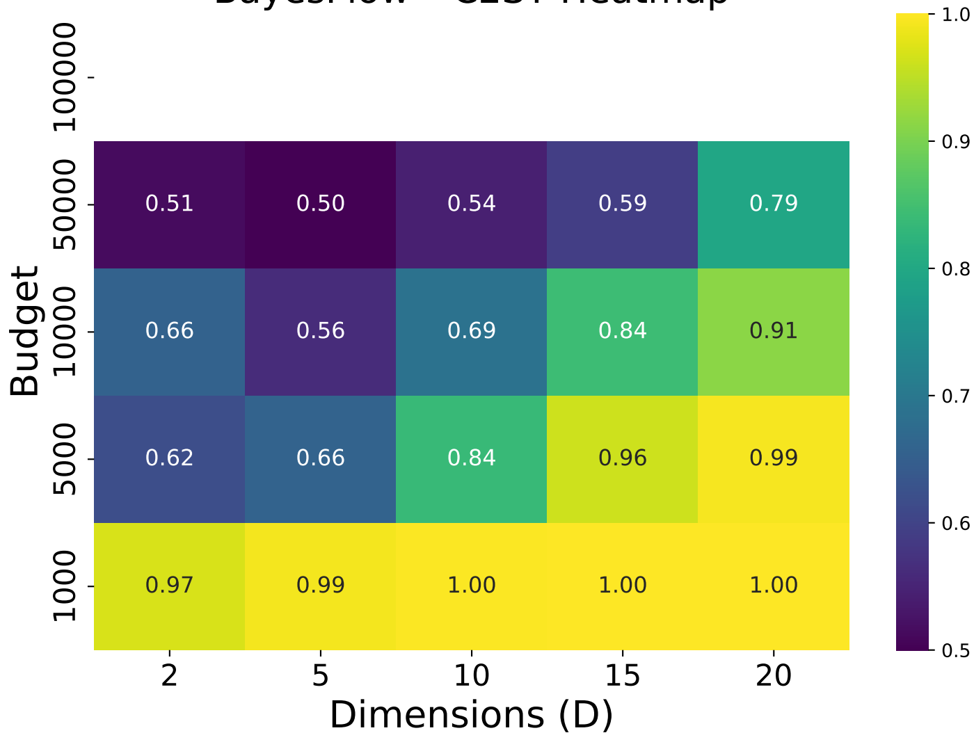
BayesFlow - C2ST Heatmap
