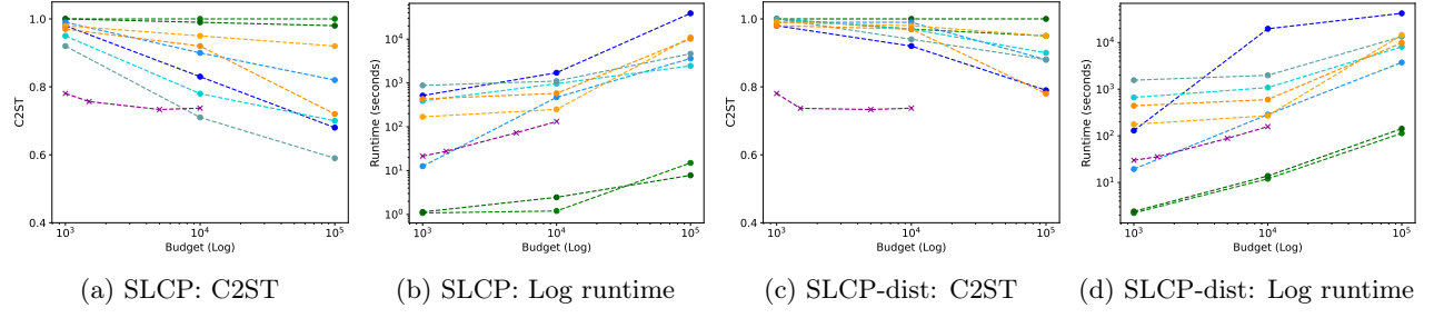
Figure 4: SLCP and SLCP with distractors benchmark results.
