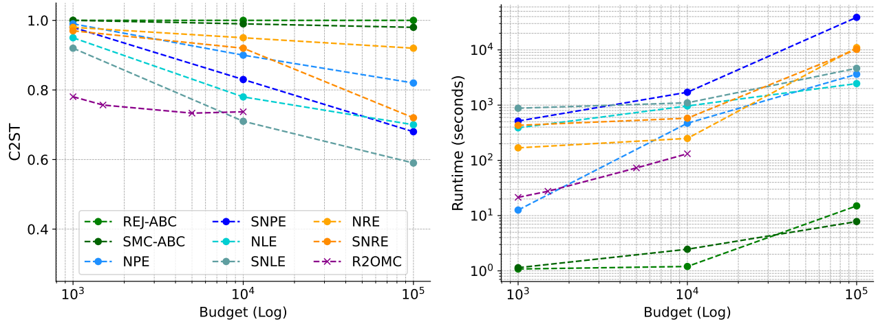
Figure 17: T.3: SLCP. From left to right: C2ST vs. budget, and runtime vs. budget.
