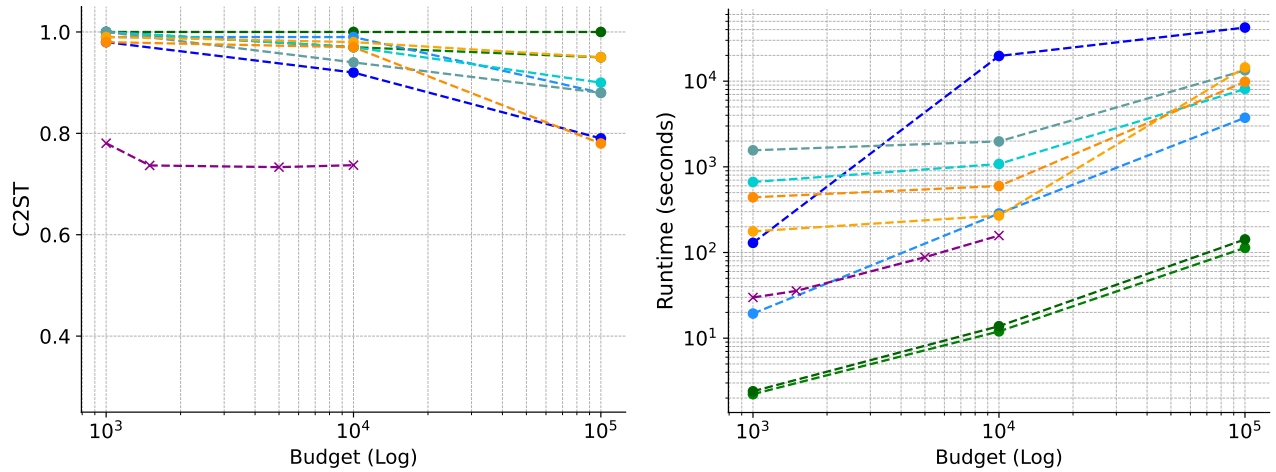
Figure 18: T.4: SLCP Distractors. From left to right: C2ST vs. budget, and runtime vs. budget.
