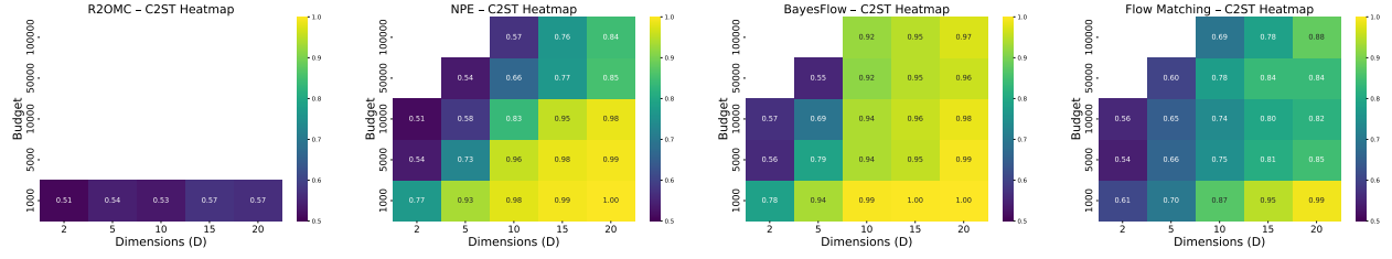
Figure 15: MoG Benchmark - MoG simulator: C2ST heatmaps for R2OMC, NPE, BayesFlow, and Flow Matching.
