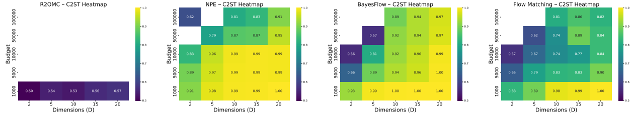
Figure 16: MoG Benchmark - MoG simulator with distractors: C2ST heatmaps for R2OMC, NPE, BayesFlow, and Flow Matching.
