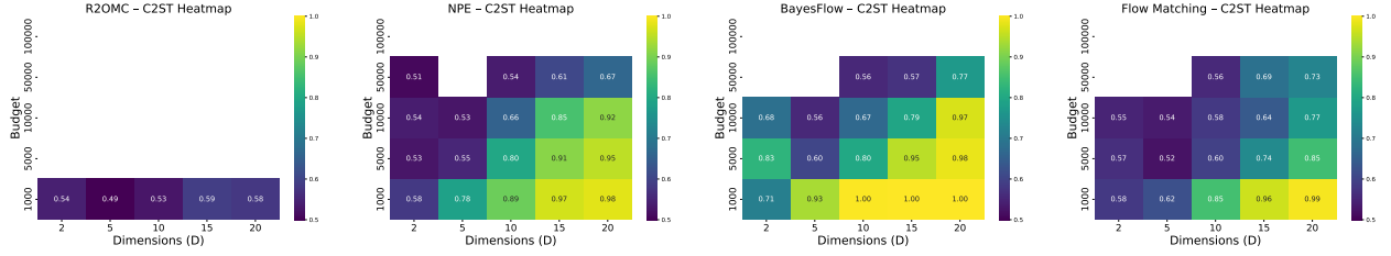
Figure 13: MoG Benchmark - Base simulator: C2ST heatmaps for R2OMC, NPE, BayesFlow, and Flow Matching.
