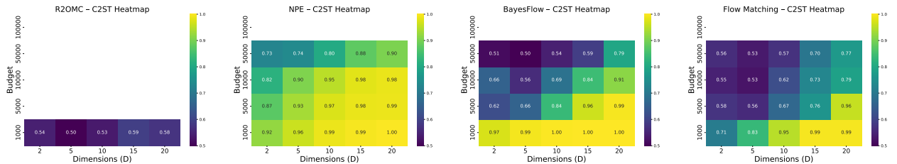
Figure 14: MoG Benchmark - Base simulator with distractors: C2ST heatmaps for R2OMC, NPE, BayesFlow, and Flow Matching.
