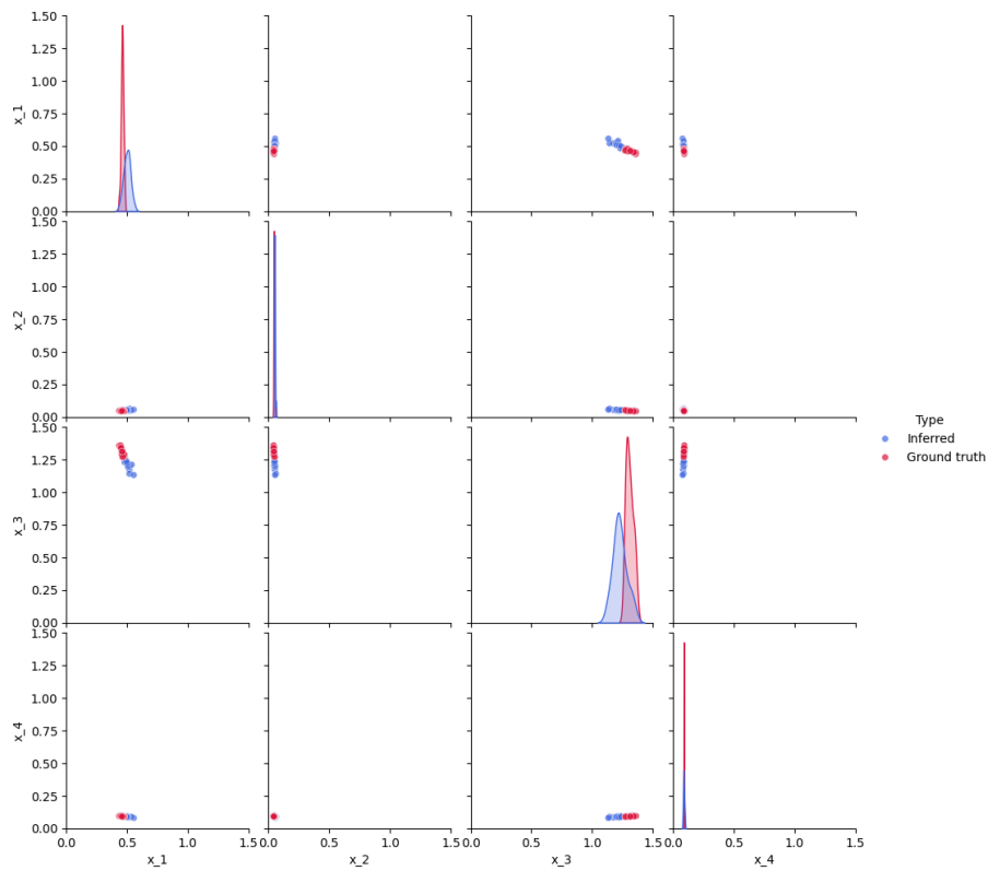
Figure 7: Lotka-Volterra model
