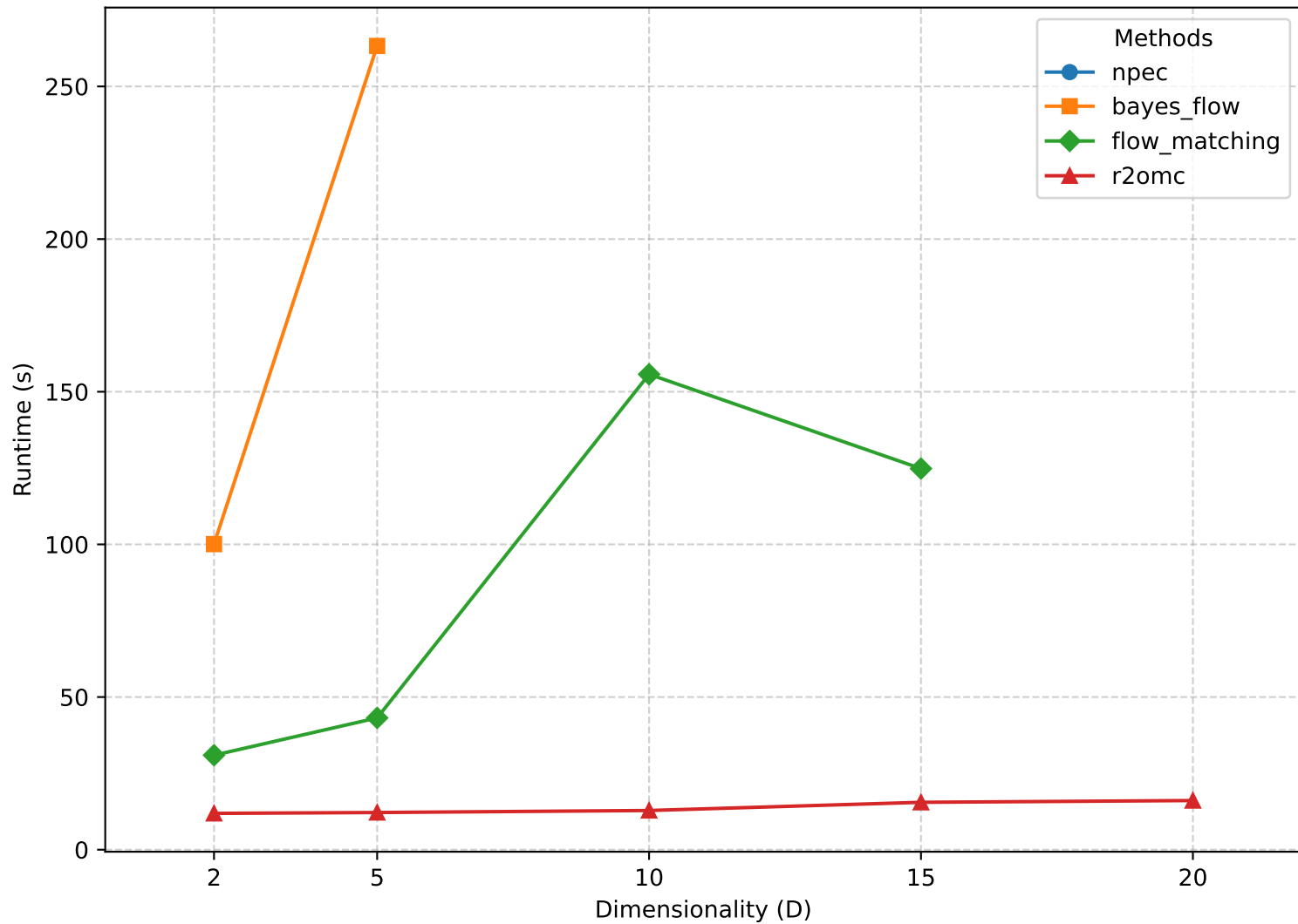
Runtime Frontier (threshold=0.8, agg=best)
