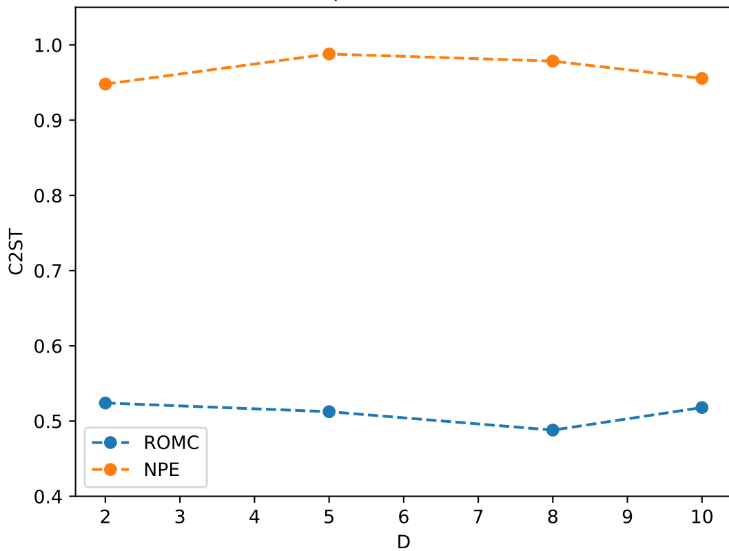
Square Gaussian
