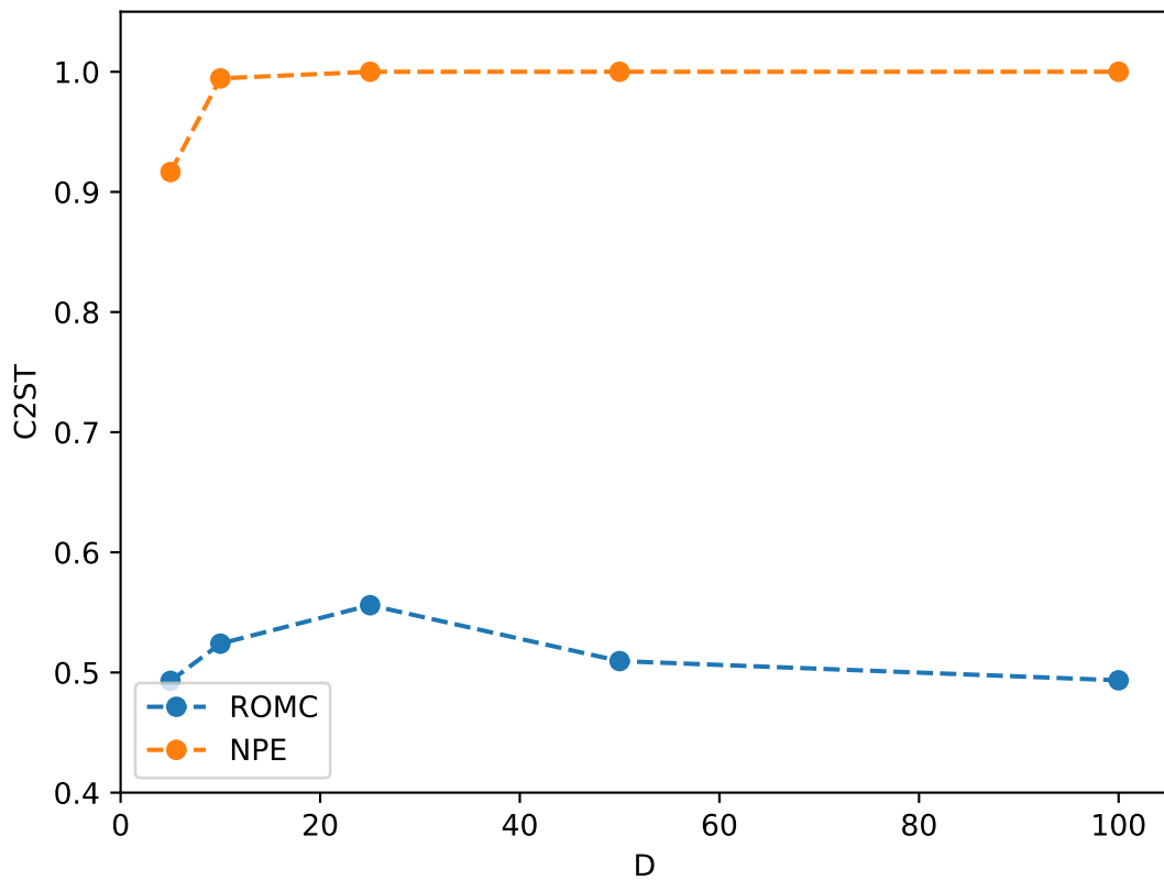
MoG (different covariances)
