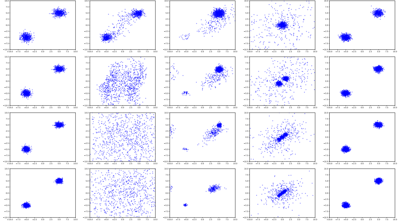
Figure 9: Multi observations MoG: Left to right: ground truth, NPE, NLE, ROMC, R2OMC. Top to bottom: N=3, N=5, N=10, N=100
