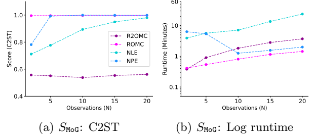
Figure 6: MoG simulator, varying nb of observations.
