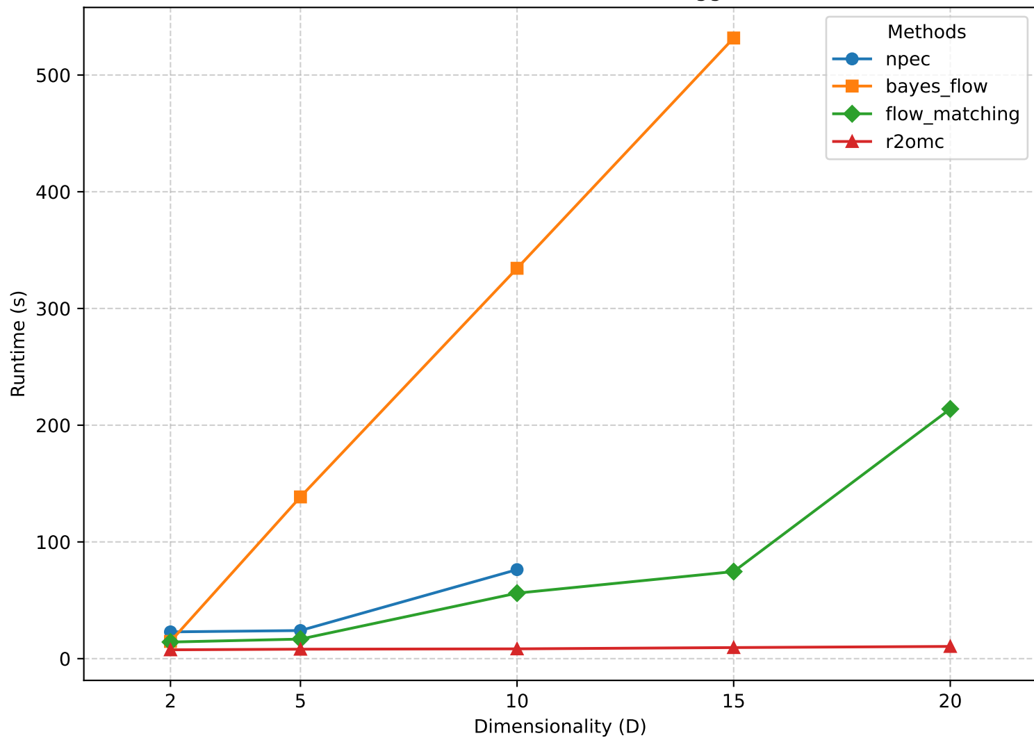
Runtime Frontier (threshold=0.8, agg=mean)
