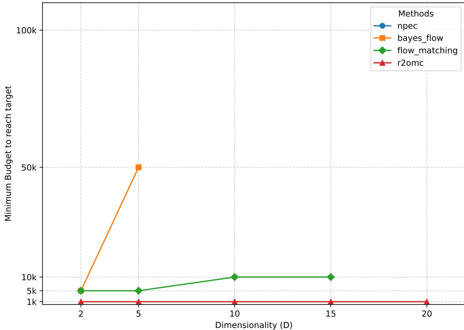
Success Frontier (threshold=0.8, agg=mean)
