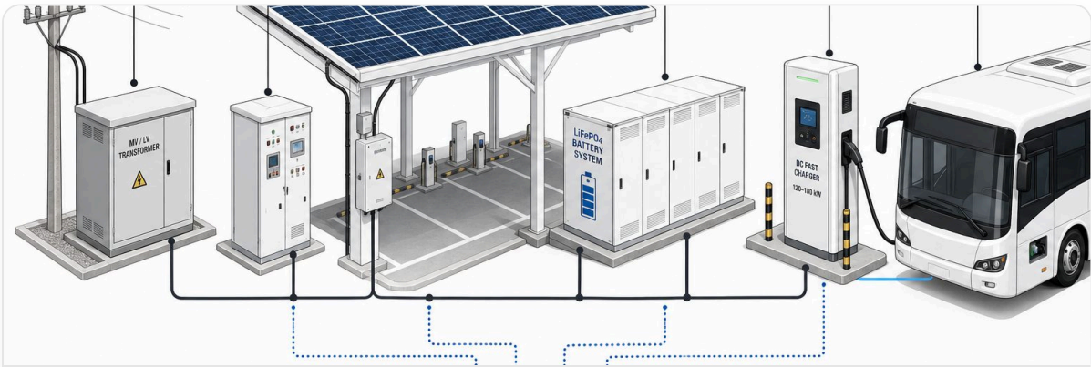
System architecture — grid, PV, storage, CCS2 dispensers and the charging management system.
