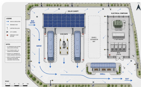
Site plan — bays, clearances, cable routes and equipment positions agreed before civils.
