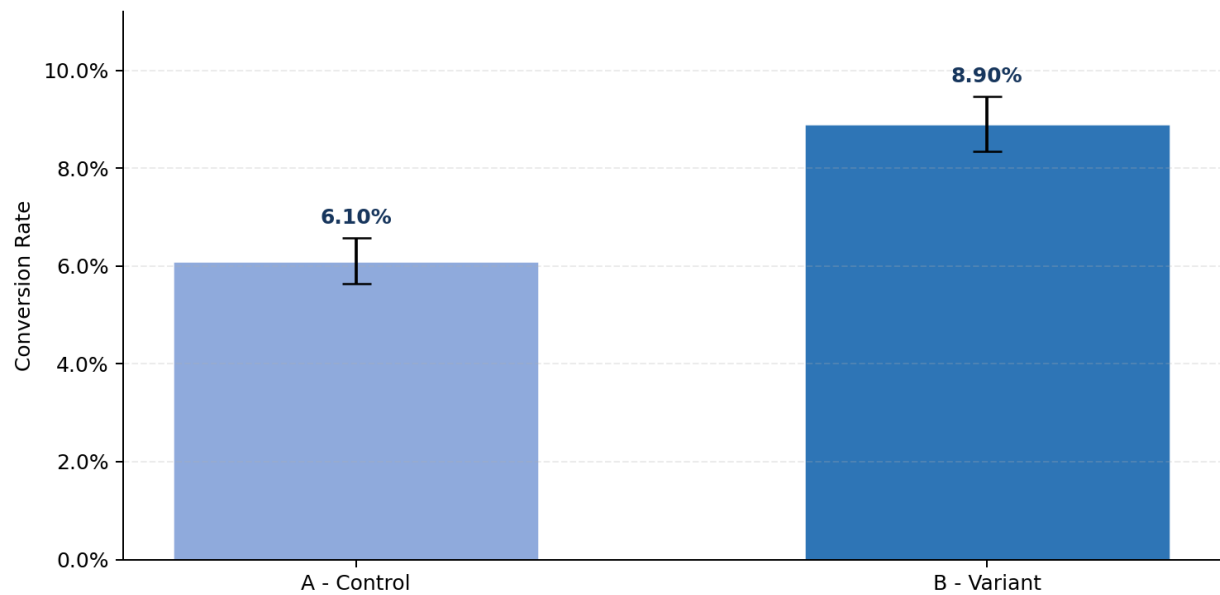
Conversion Rates with 95% Confidence Intervals
