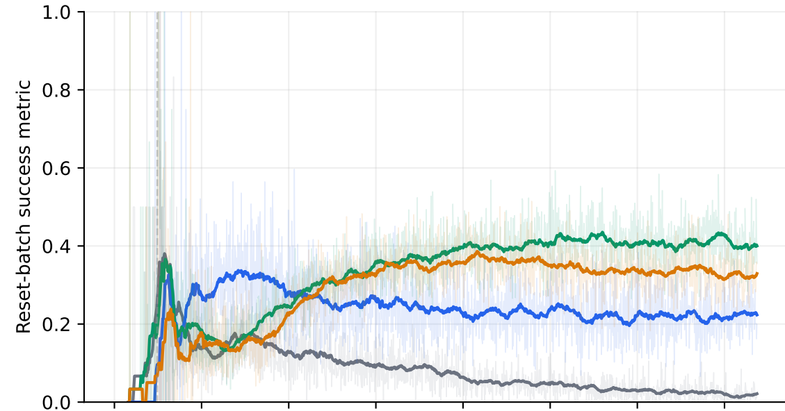
Plug insertion · seed 0 · raw traces and 30-update moving means
