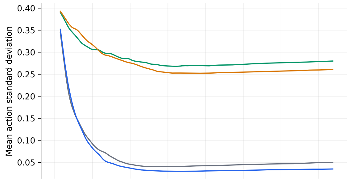
Optimization diagnostics · seed 0
