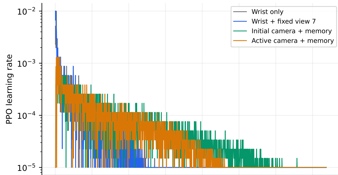
Optimization diagnostics · seed 0
