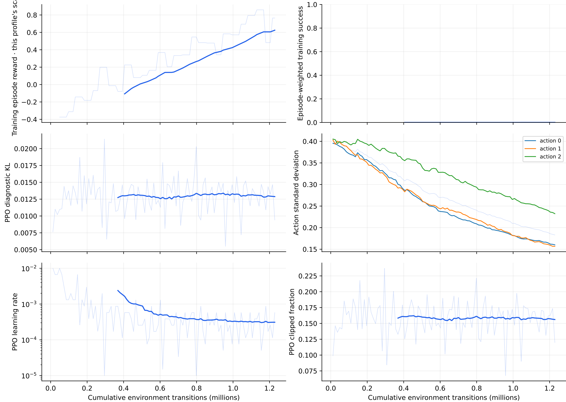
Corrected-training reward profile: progress · seed 0 · 100 recorded updates
