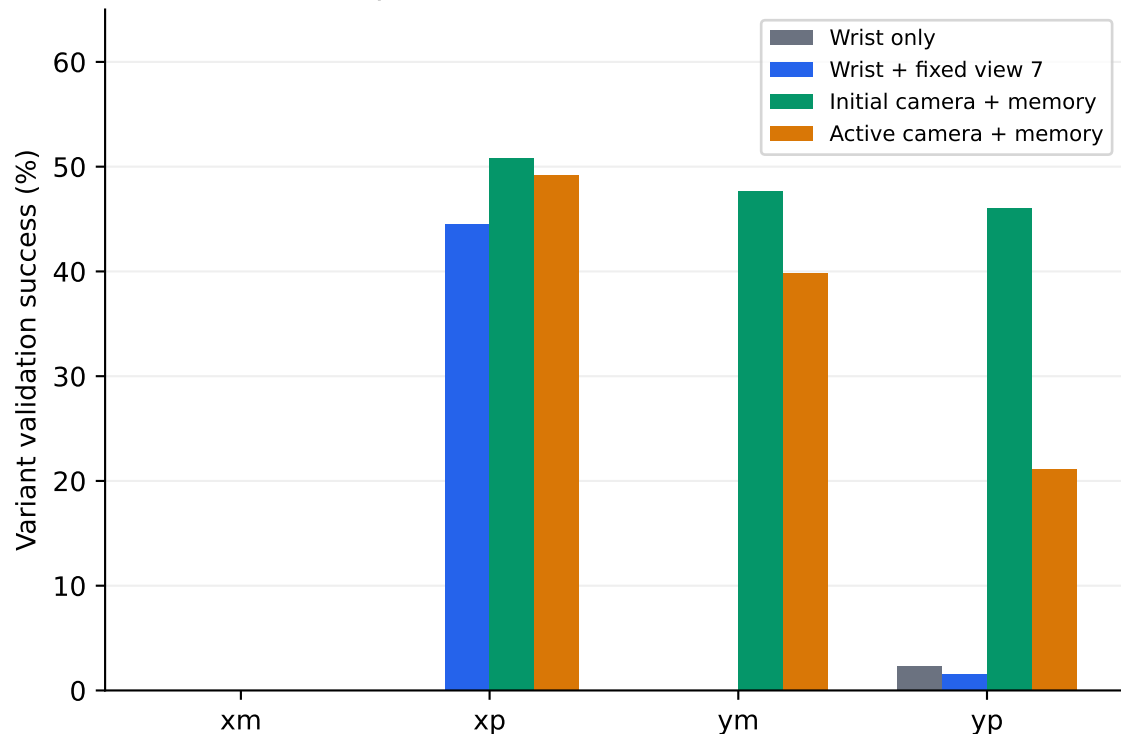
128 episodes / variant · no xm successes
