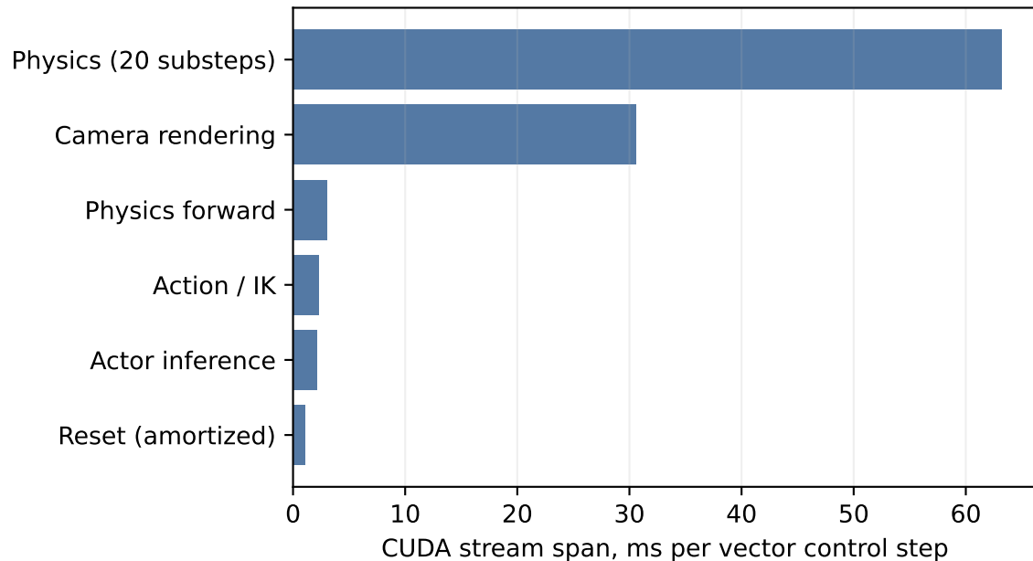
Active / N512 rollout attribution Instrumented; excludes PPO updates
