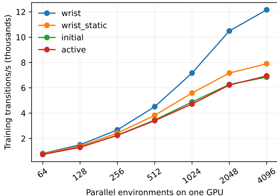
Full PPO: rollout + optimization 12 iterations, first 3 excluded
