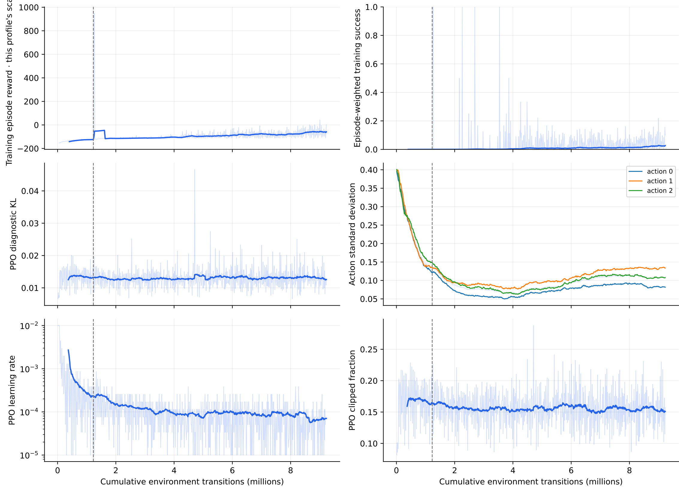
Corrected-training reward profile: legacy_log_hold · seed 0 · 751 recorded updates
