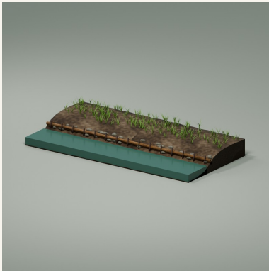
Backwater bank with coir protection
