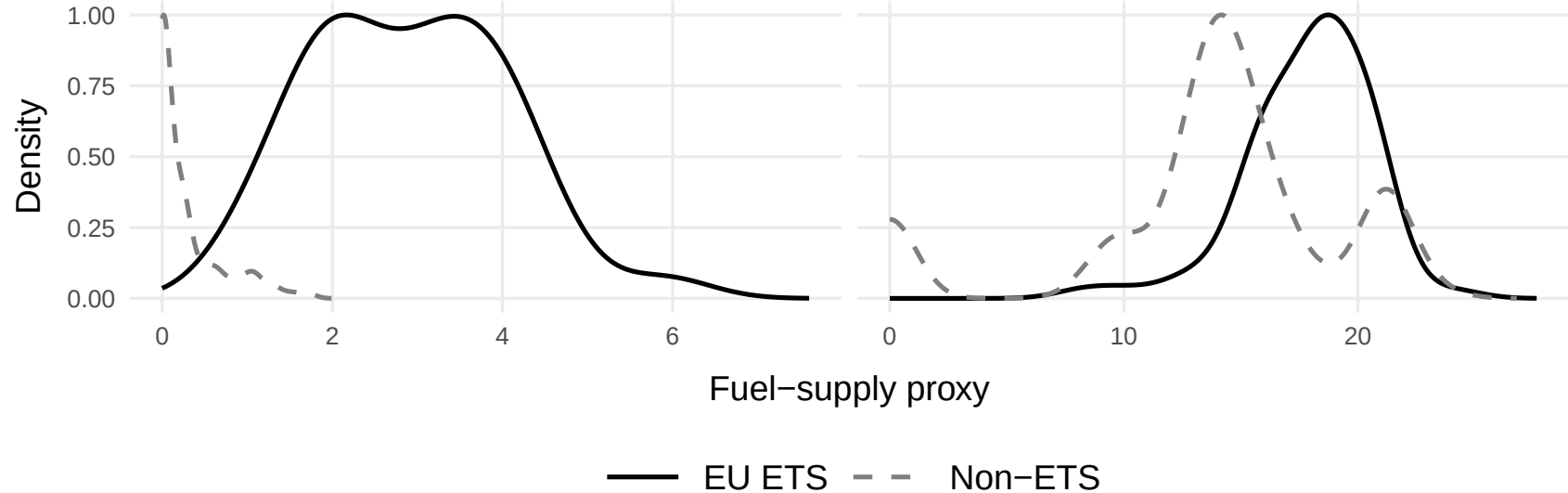
B2B proxy
