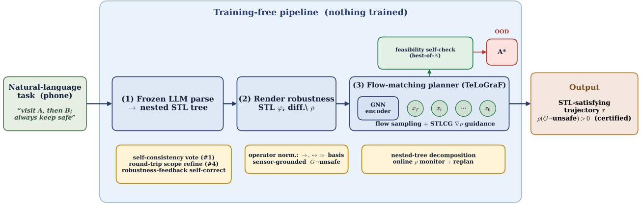
Figure 1: The NL2TL-Tree pipeline (everything frozen / training-free). Five stages—mobile NL, few-shot-prompted LLM parse into a nested STL tree, rendering to differentiable robustness \rho , a frozen flow-matching planner (TeLoGraF) with STLGG guidance, and the executed trajectory—each annotated with the test-time mechanisms it uses (§4); the feasibility self-check routes out-of-distribution specs to an A^* fallback.
