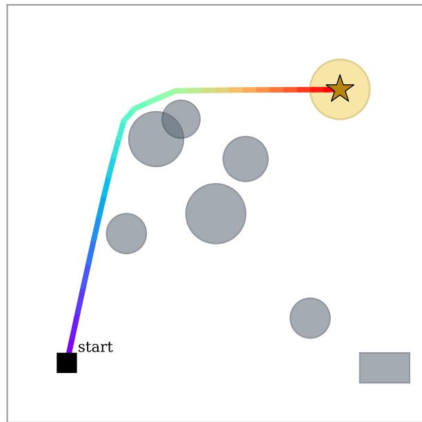
(a) reach_within_T TeLoGraF (flow + STL CG)
