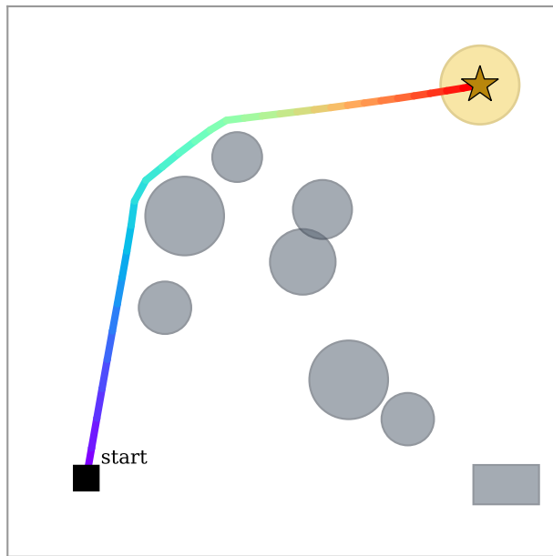
(b) reach_avoid TeLoGraF (flow + STL CG)
