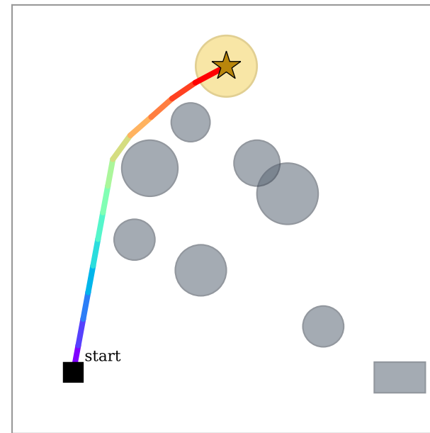
(c) reach_goal_north TeLoGraF (flow + STL CG)
