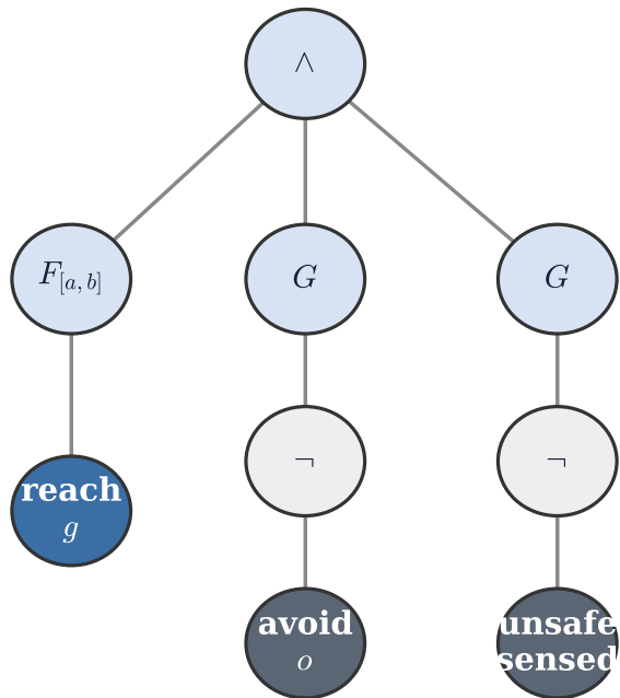
(a) Nested STL spec
