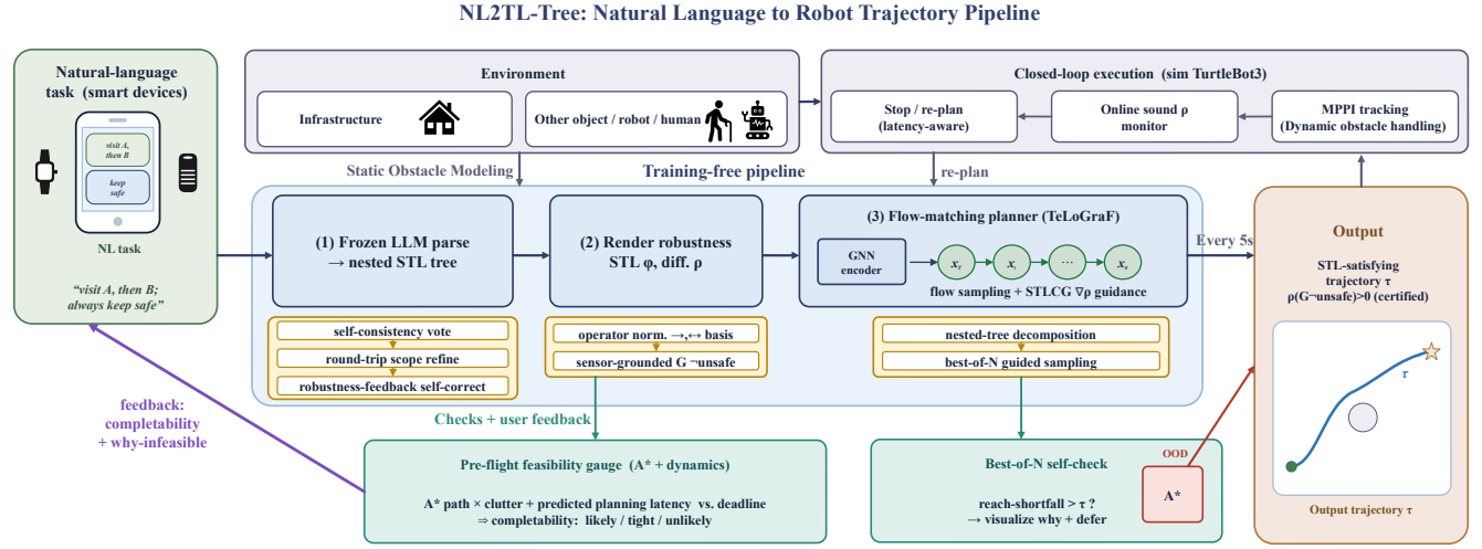
Figure 1: The NL2TL-Tree pipeline: everything frozen / training-free. A smart-device task is parsed by a frozen LLM into a nested STL tree, rendered to a differentiable robustness \rho , and planned by a frozen flow-matching planner (TeLoGraF) under STLCG gradient guidance. The trajectory executes closed-loop on a simulated TurtleBot3: the planner models sensed obstacles statically , a reactive MPPI tracker avoids the live -sensed field, and an online sound- \rho monitor triggers latency-aware stop/re-plans. Each stage is annotated with its test-time mechanisms (§4); a checks-and-feedback layer returns the completability and a why-infeasible explanation to the user.
