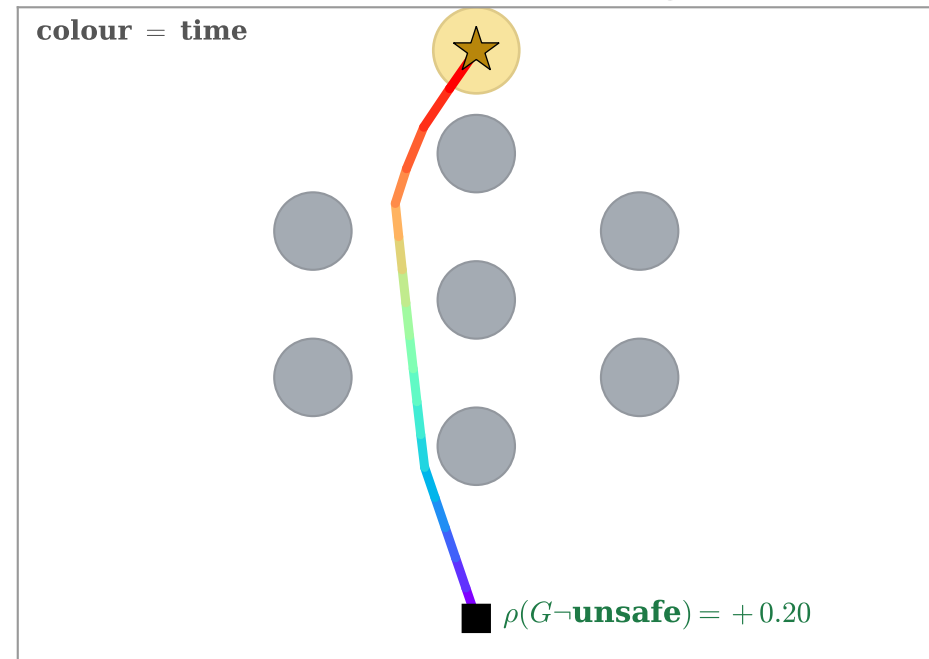
(c) Real flow plan slaloming a cluster
