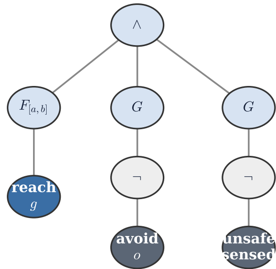
(a) Nested STL spec
