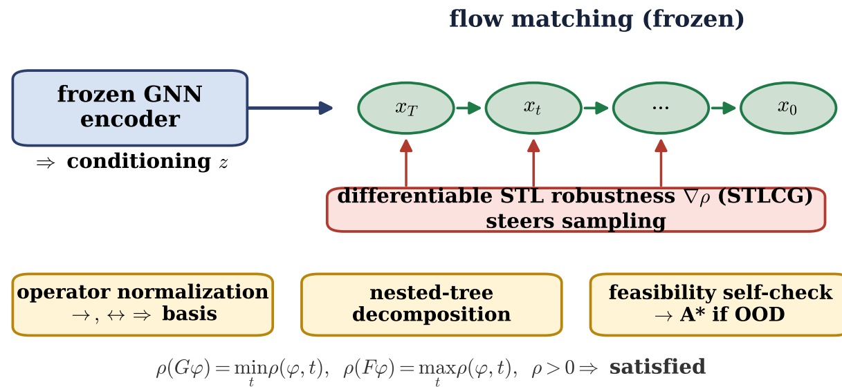
(b) Frozen flow-matching planner + robustness guidance
