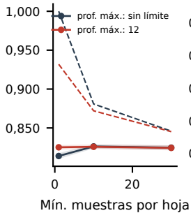
Random Forest
