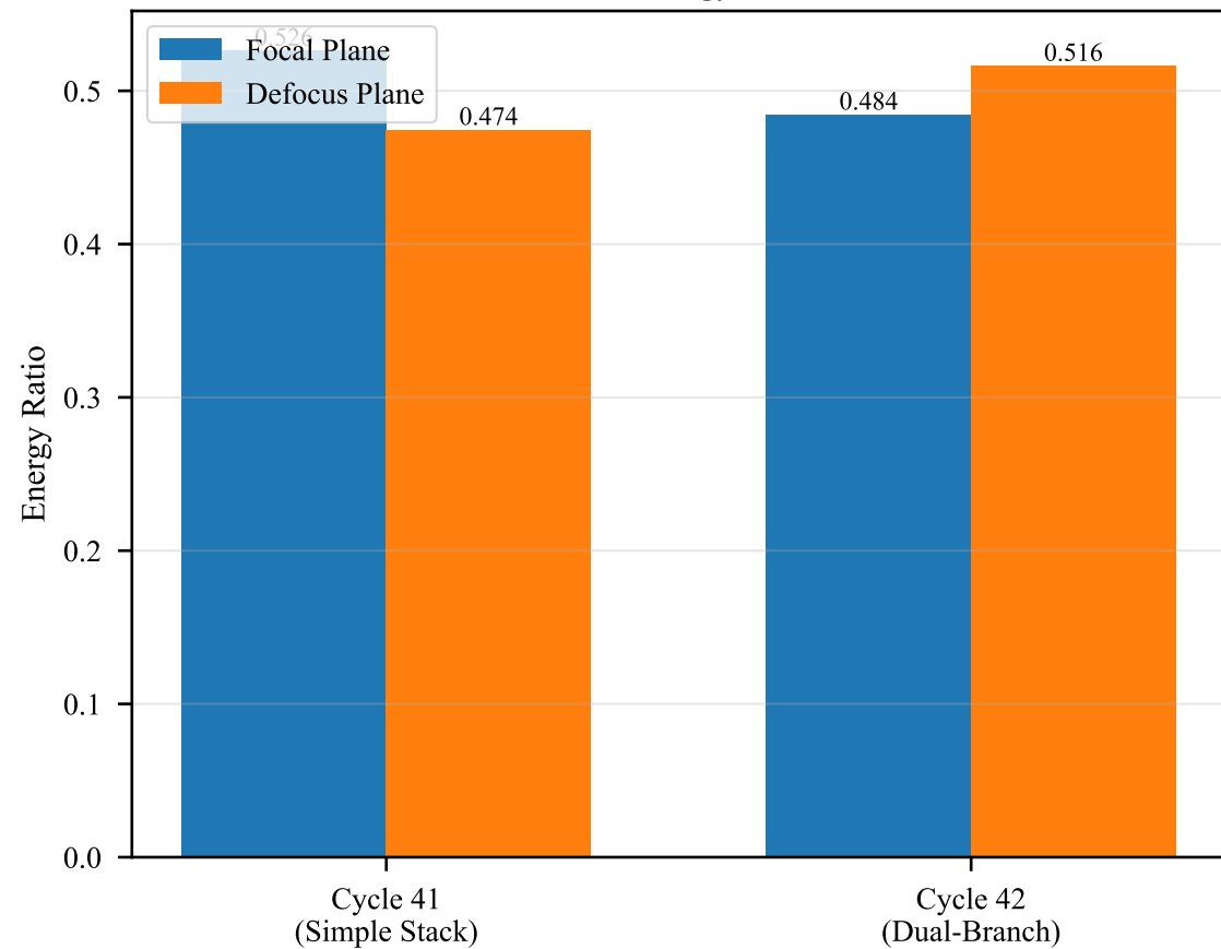
(a) Gradient Energy Distribution
