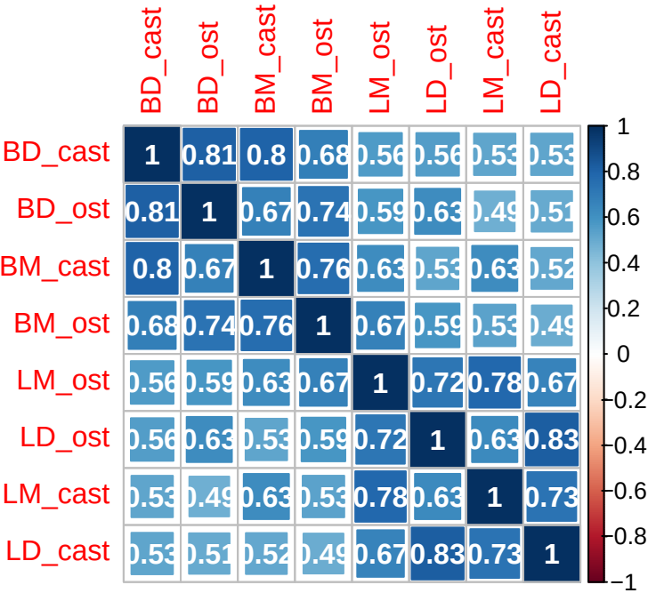
Spearman correlations
