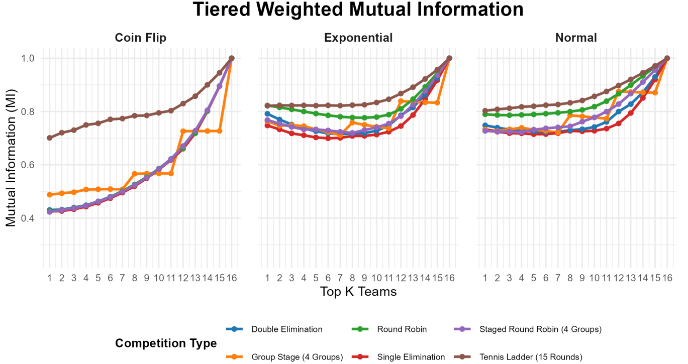
Figure 2: Tiered weighted mutual information of various competition structures as a function of the top K teams for three distributions of true strengths (Coin Flip, Exponential, Normal).
