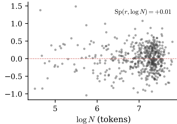
TwoNN dim
