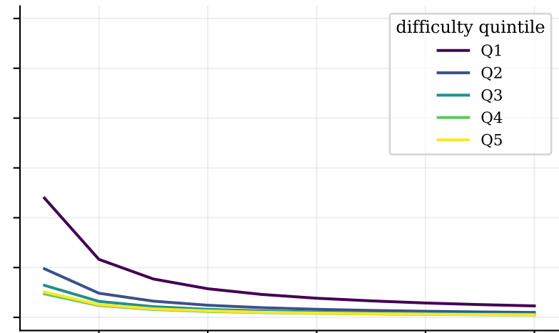
Phi-4-R
