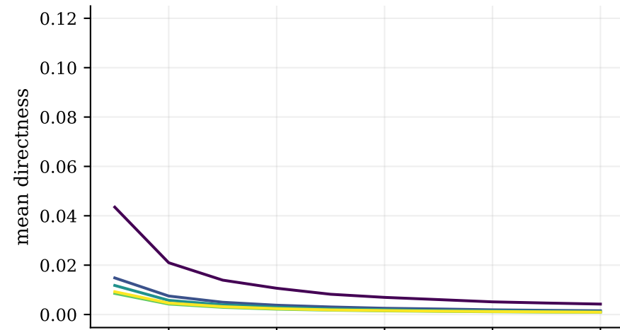
R1-Llama-8B
