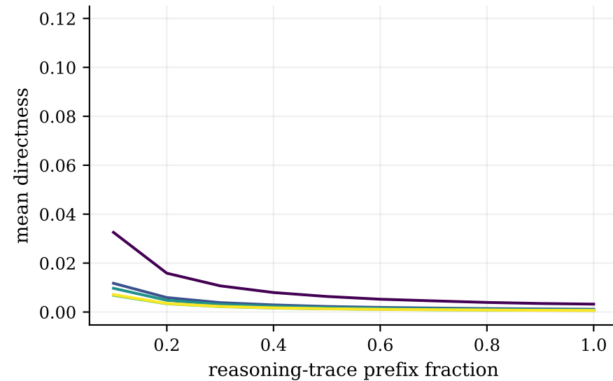
R1-Llama-8B
