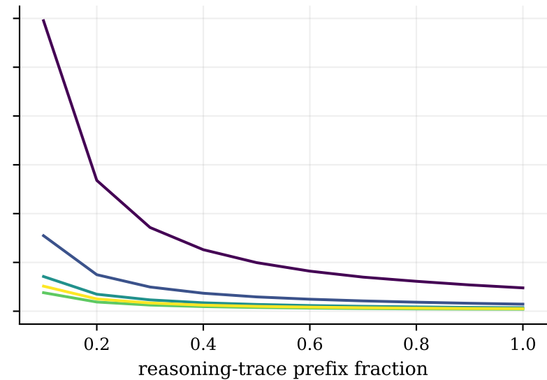
Phi-4-R
