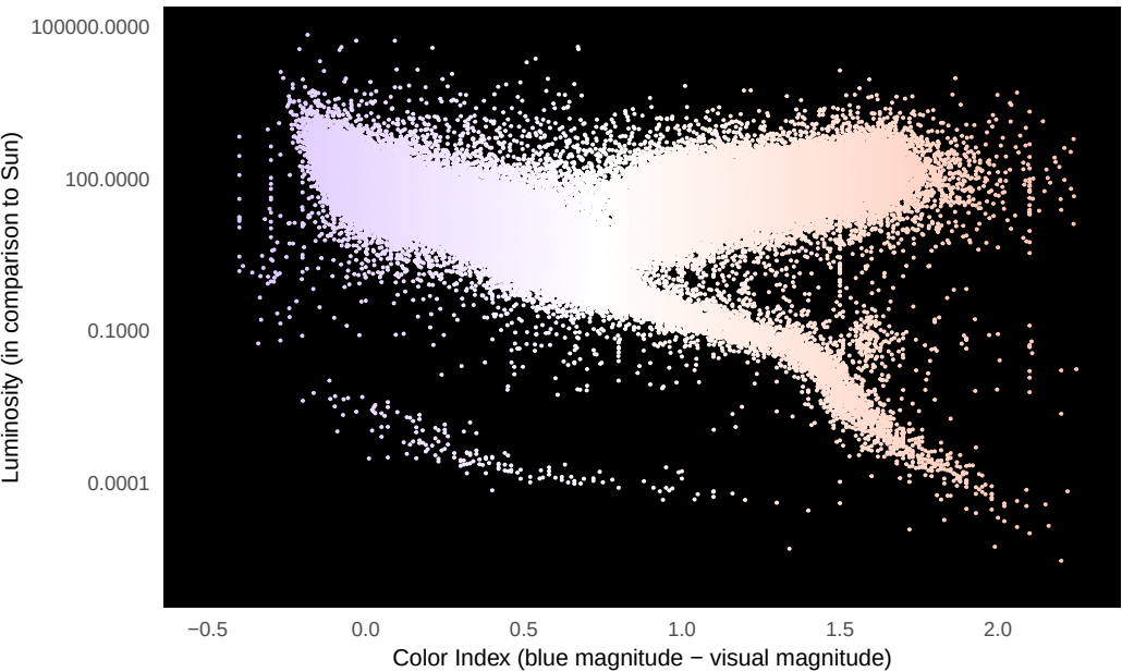
Hertzsprung–Russell Diagram
